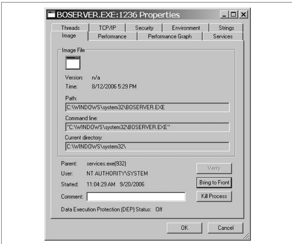
Figure 21-7. The Process Explorer Process Properties window
