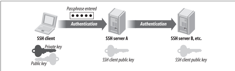
Figure 15-6. Agent forwarding
