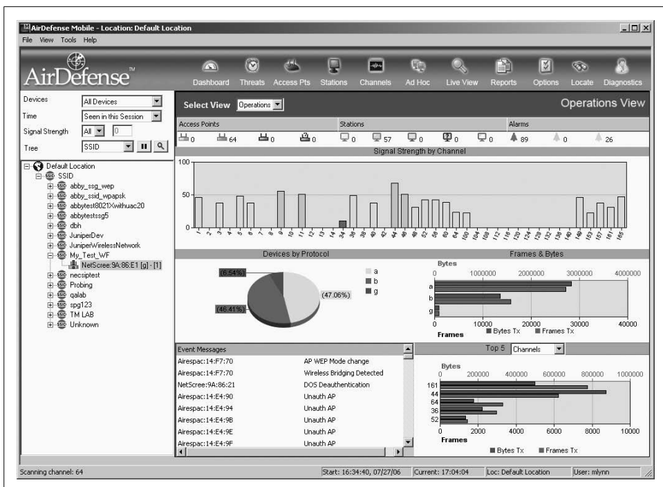
Figure 5-11. The AirDefense Mobile interface
