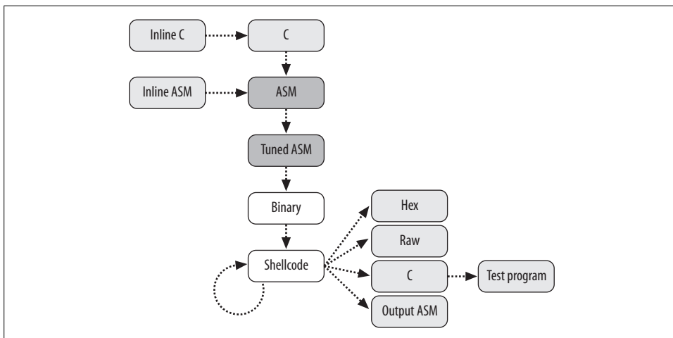
Figure 10-2. ShellForge's architecture
